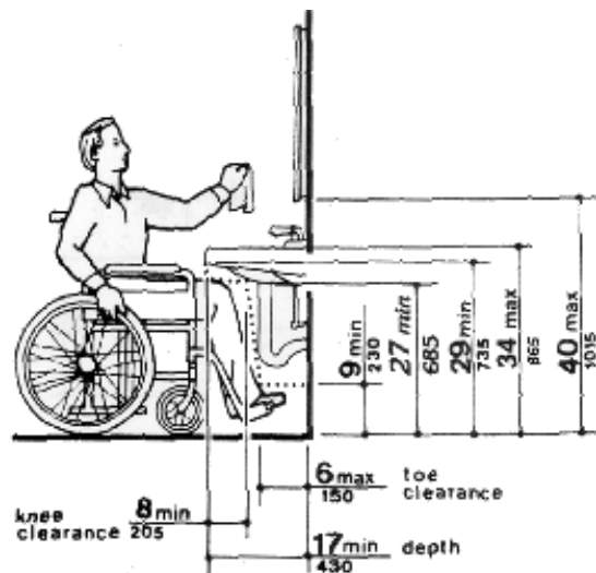
Fig. 31 Lavatory Clearances
