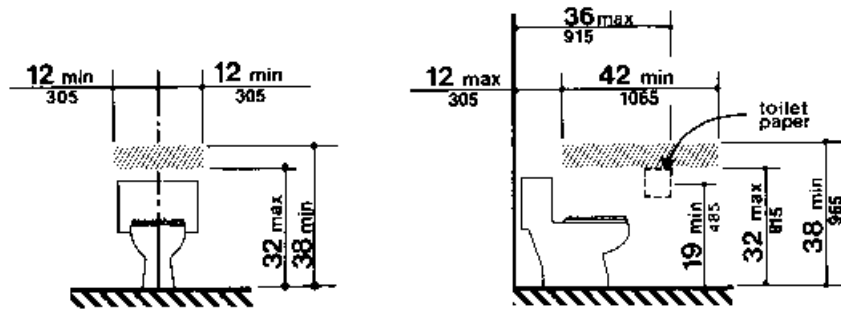
Reinforced Areas for Installation of Grab Bars
